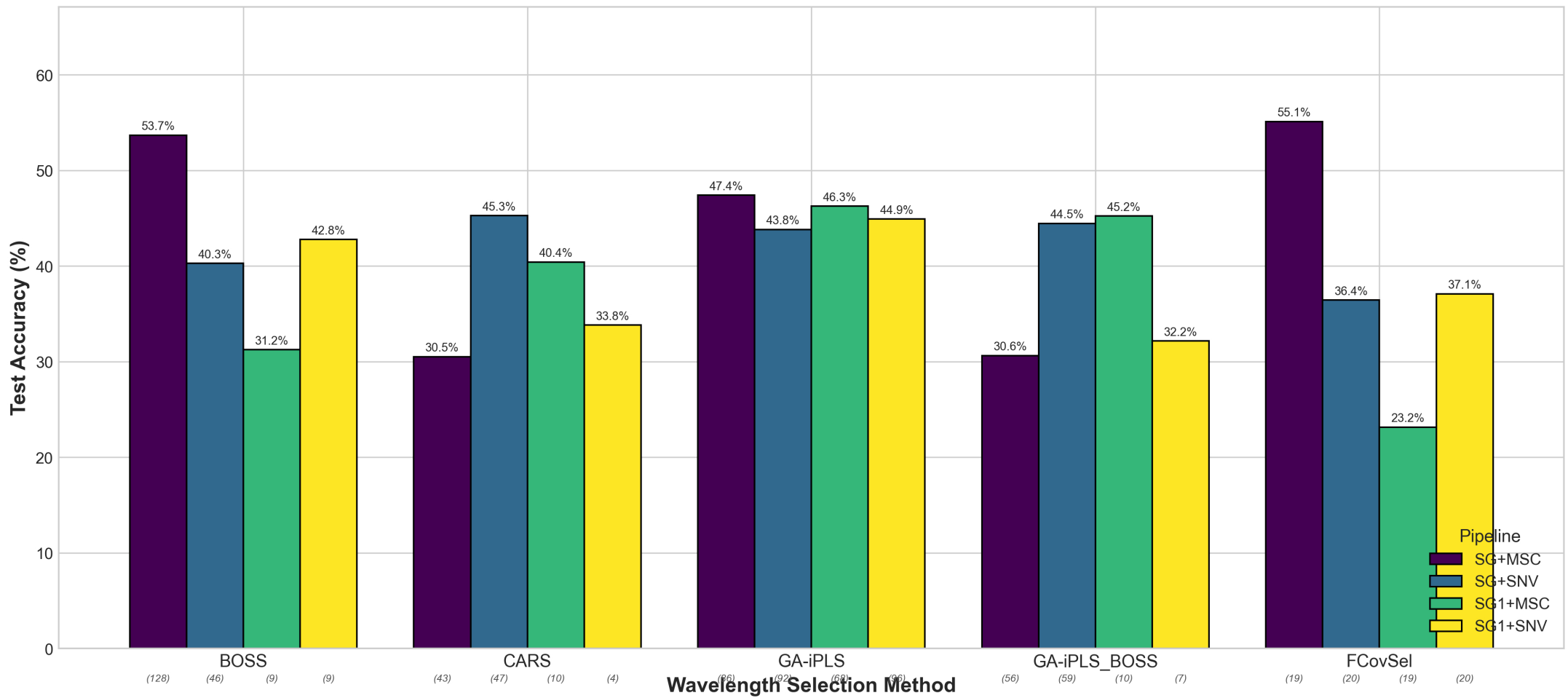
3D-CNN Test Accuracy by Wavelength Selection Method & Preprocessing (Indian Pines) (Number of selected bands shown in parentheses)
